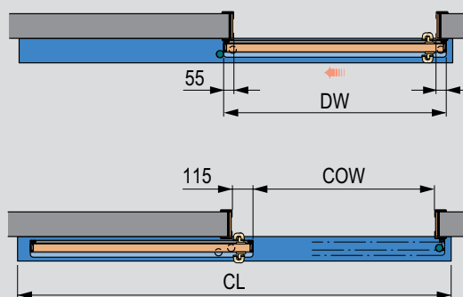
ASSA ABLOY Hermetic-L Left opening shown, right opening mirror image
